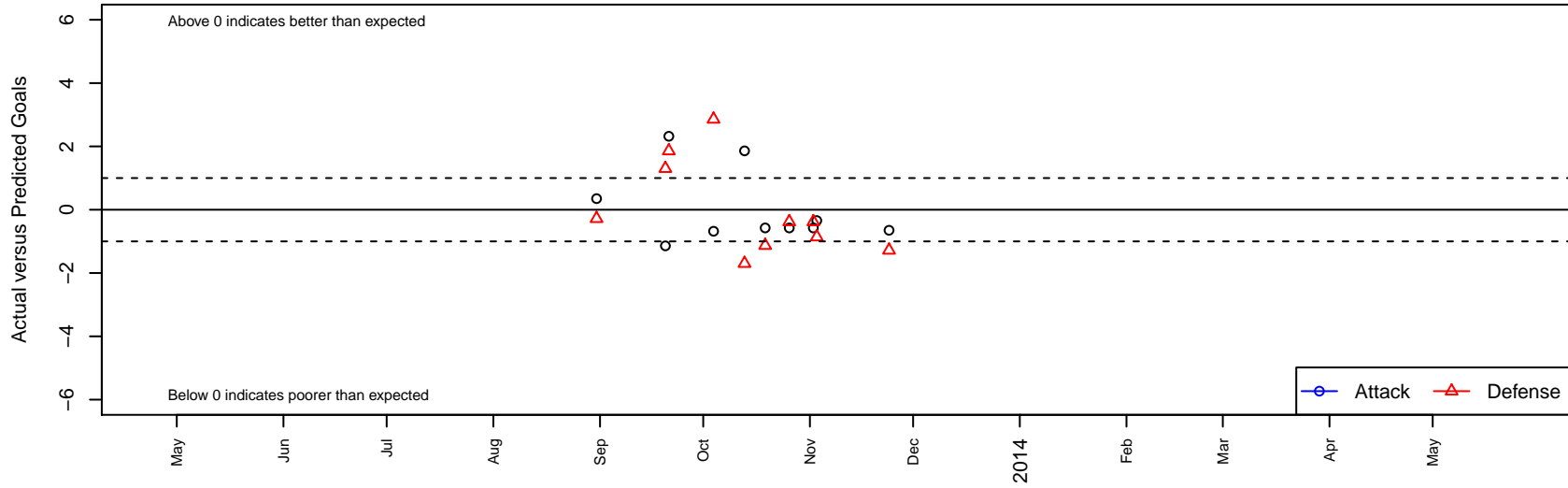
Briceno SC Earthquakes G00 Dots are actual minus expected GF (blue circles) and GA (red triangles). Blue line is smoothed change in attack strength. Red is smoothed change in defense strength.
